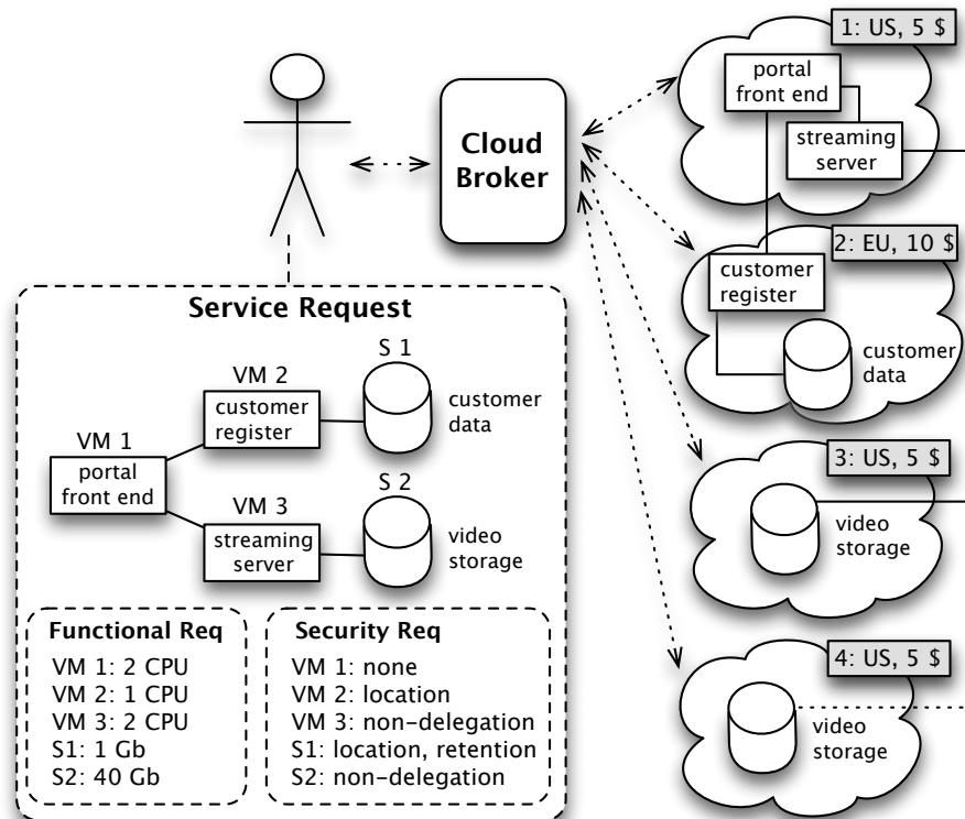
Figure 2: A Cloud Broker negotiating security requirements
